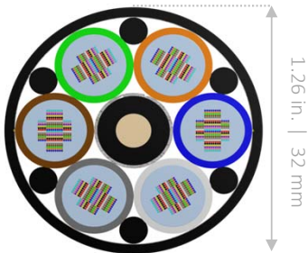
Largest Stranded Tube 1,728 Fibers
