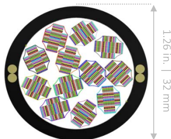
Extreme Density 3,456 Fibers
