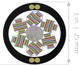
Extreme Density 1,728 Fibers
