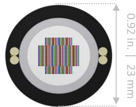
Largest Central Tube 864 Fibers
